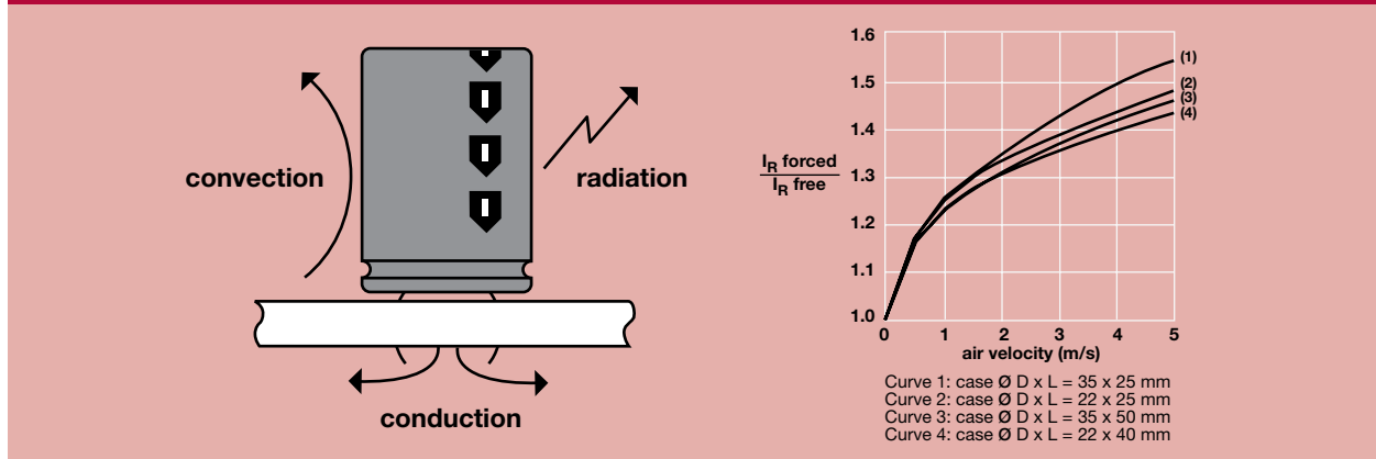
Figure 8. Transport of Heat from the Aluminum Capacitor to its Environment and the Effect of Airflow
