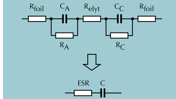
Figure 3. Equivalent AC Circuit
