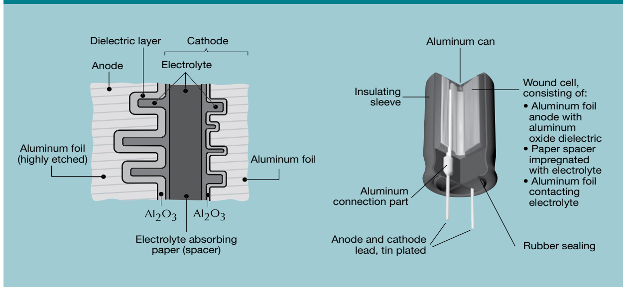
Figure 2. Basic Construction of Non-Solid Aluminum Capacitors
