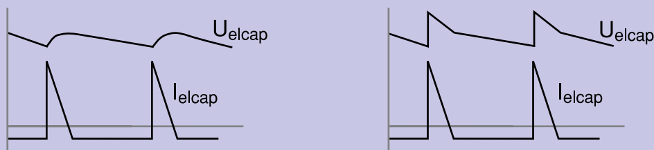
Figure 9. Voltage Ripple on Aluminum Capacitors without and with ESR
