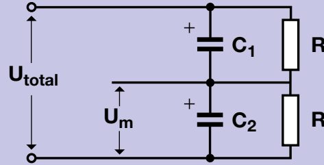
Figure 10. Balancing Resistors
