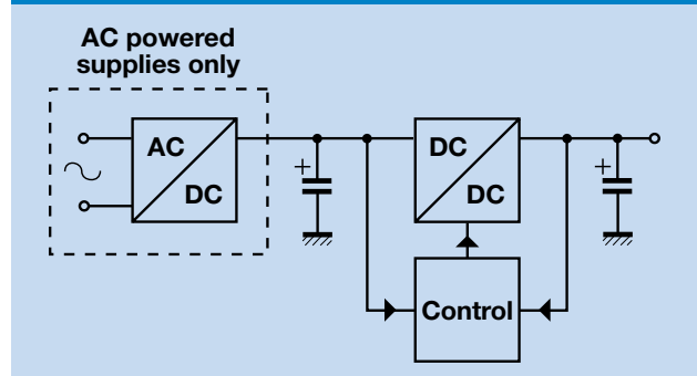
Figure 1. Basic Topology of a Power Supply
