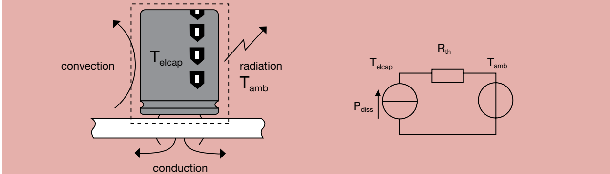
Figure 6. A simple thermal model
